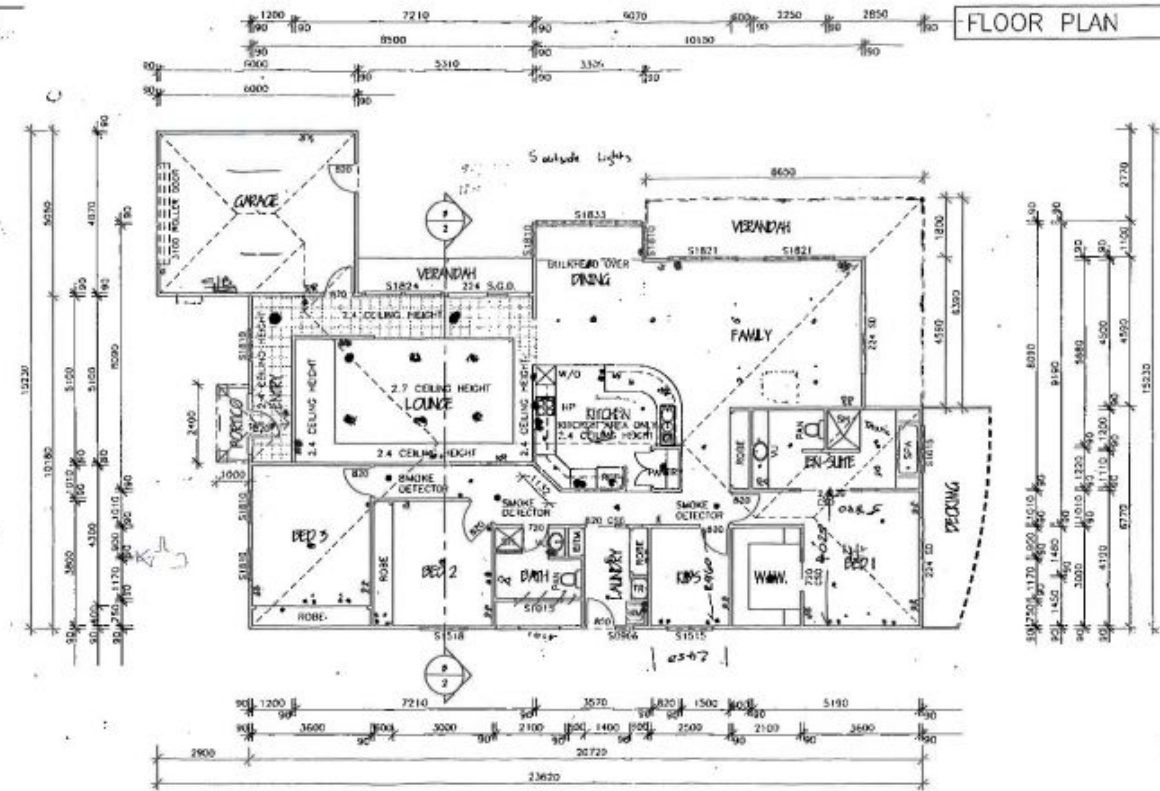
PROPOSED FLOOR PLAN 1:100
